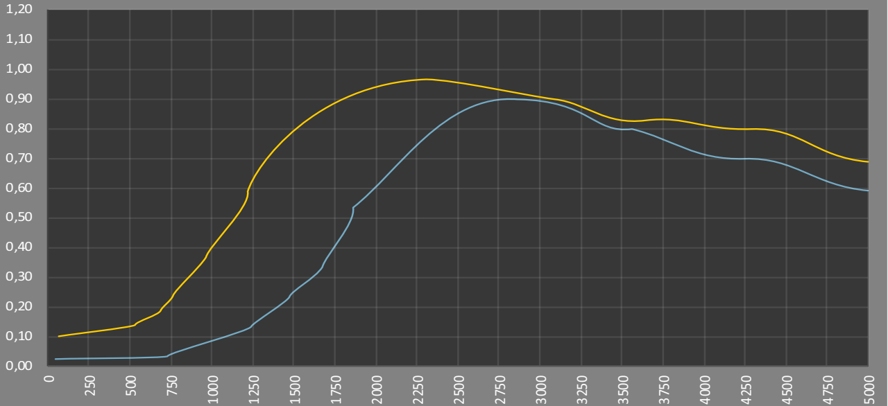
Absorption chart ISO 11654 - ISO354
